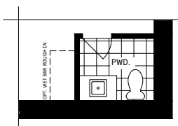
6 Finished Basement Powder Room
