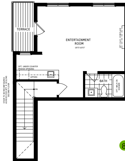
5 Loft Entertainment Room
