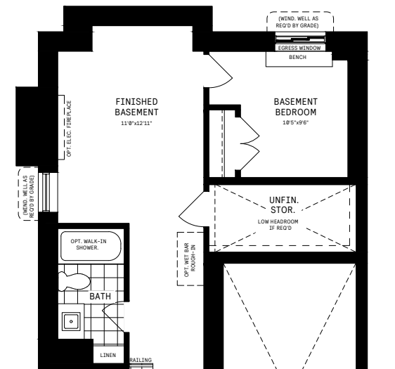
8 Finished Basement Package
